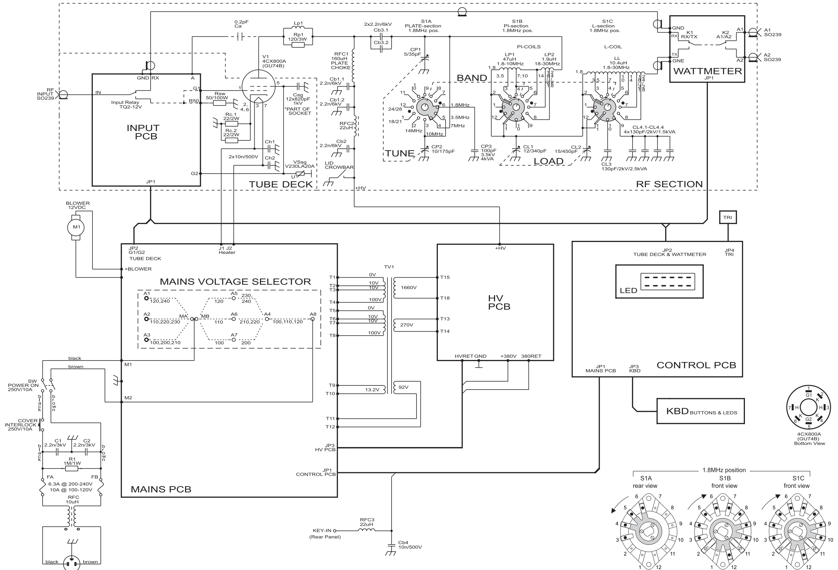
Fig. 5-1 ACOM1010 Simplified Schematic Diagram
